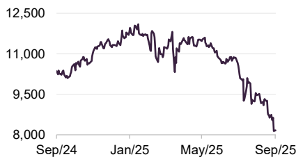
Figure 10: LSEG (GBP)
