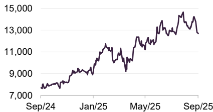
Figure 9: Nintendo (JPY)
